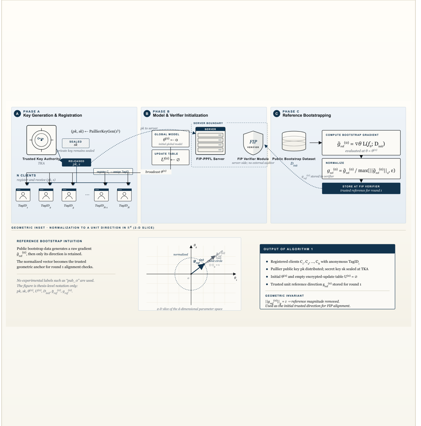
Figure 1. Algorithm 1. The TKA generates the Paillier key pair and keeps sk sealed while releasing only pk and the fixed-point scale S . The server initializes \theta^{(0)} \leftarrow \text{InitModel}(f_\theta) (zero initialization for the logistic-regression experiments) together with U^{(0)} = \emptyset , broadcasts \theta^{(0)} to the registered clients, and the server-side FIP Verifier stores the initial trusted reference direction. The trusted public bootstrap set D_{\text{init}} produces the raw gradient \tilde{g}_{\text{ref}}^{(0)} , which is normalized to g_{\text{ref}}^{(0)} using \max(\|\tilde{g}_{\text{ref}}^{(0)}\|_2, \epsilon) . The bottom inset shows the geometric normalization from a raw gradient vector to a unit direction in a 2-D slice of the parameter
